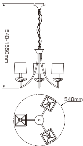
AKIRA 0783 ■ cromo brillo ■ polished chrome ⚡ 3 x 40W E14 (no inc.)
